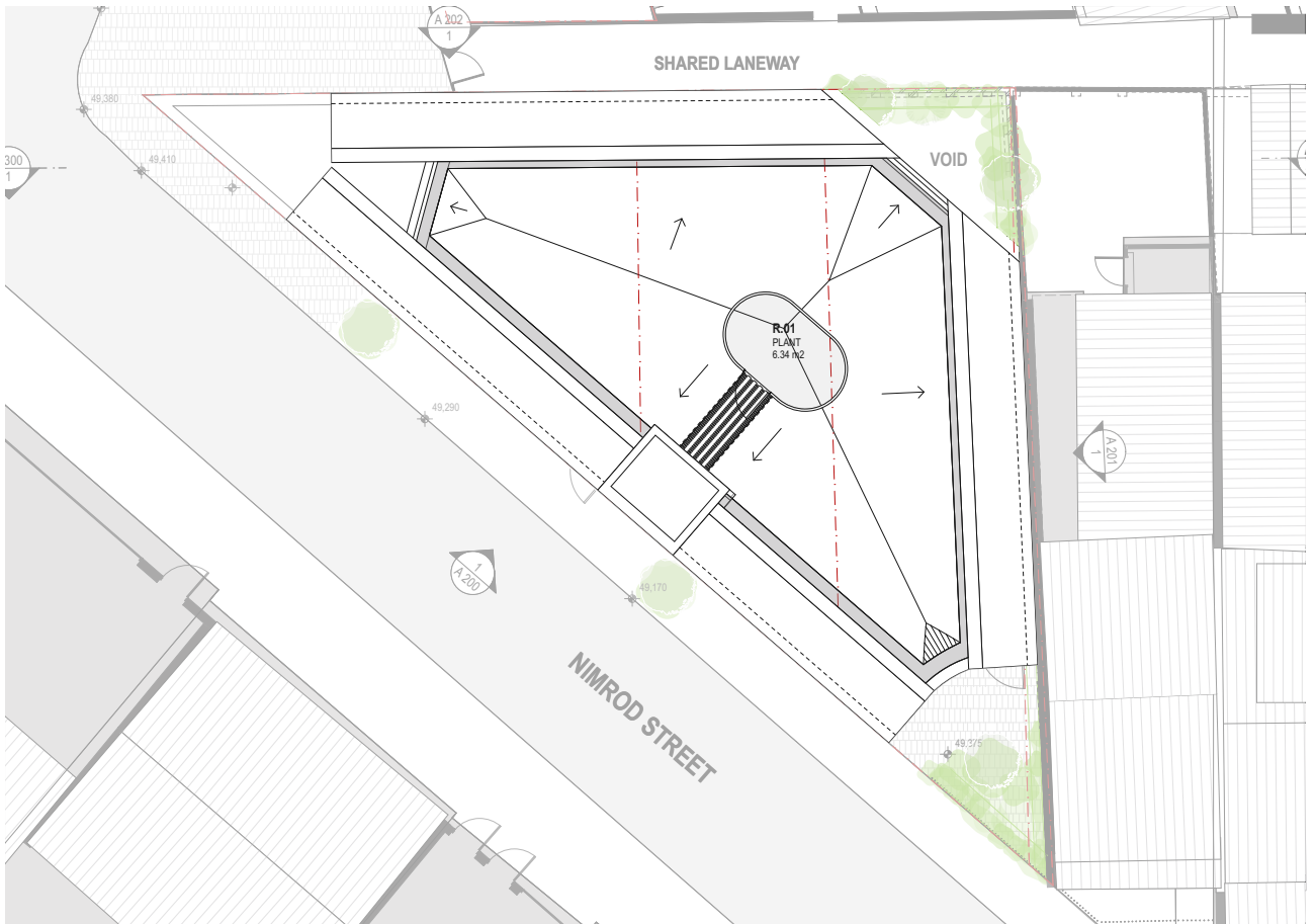
Figure 174: Roof Plan. Source: TZG Architects, 2022.
