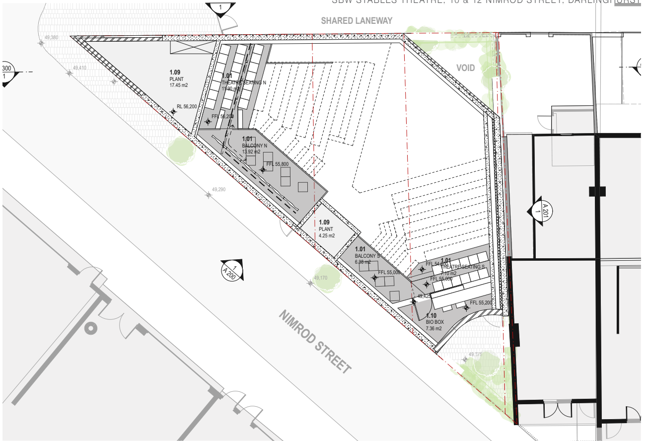
Figure 173: Level 1 - Upper Theatre Plan. Source: TZG Architects, 2022.
