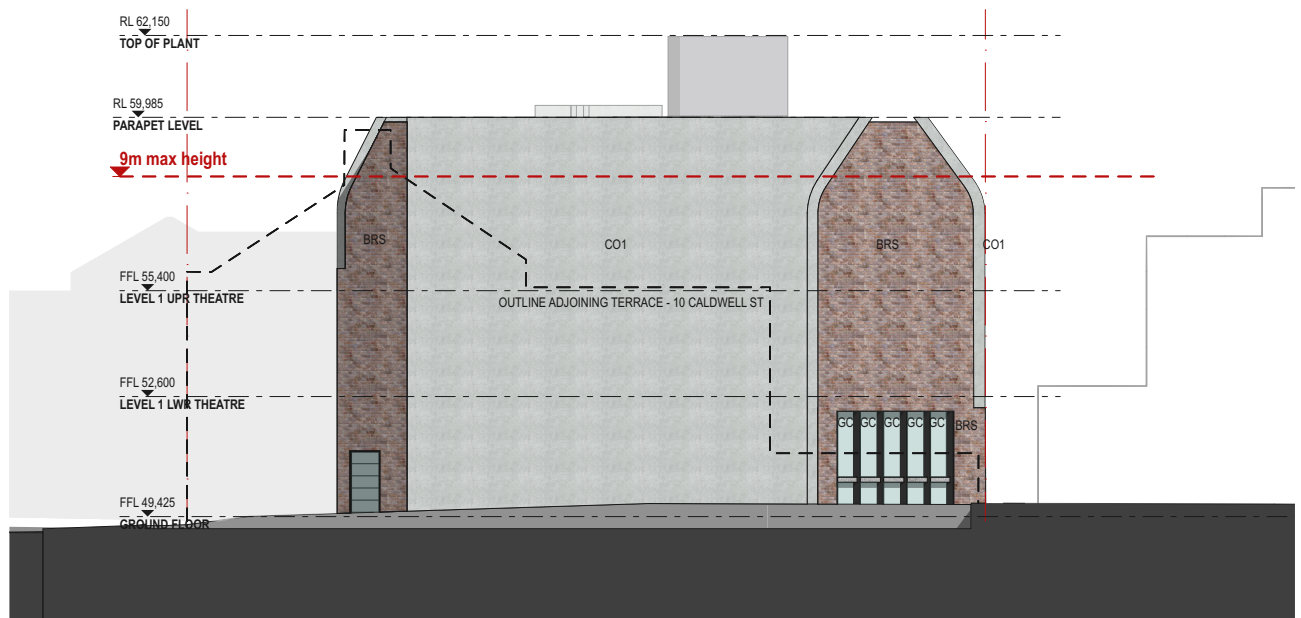
Figure 176: East Elevation - Terraces. Source: TZG Architects, 2022.
